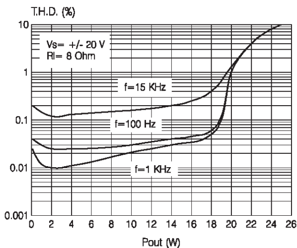
Figure 7: T.H.D. vs. Output Power
